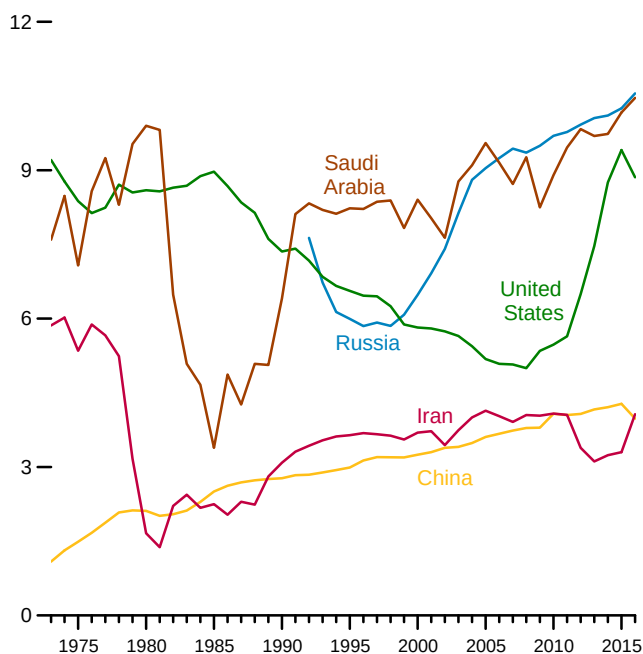
Selected Producers, 1973–2016
