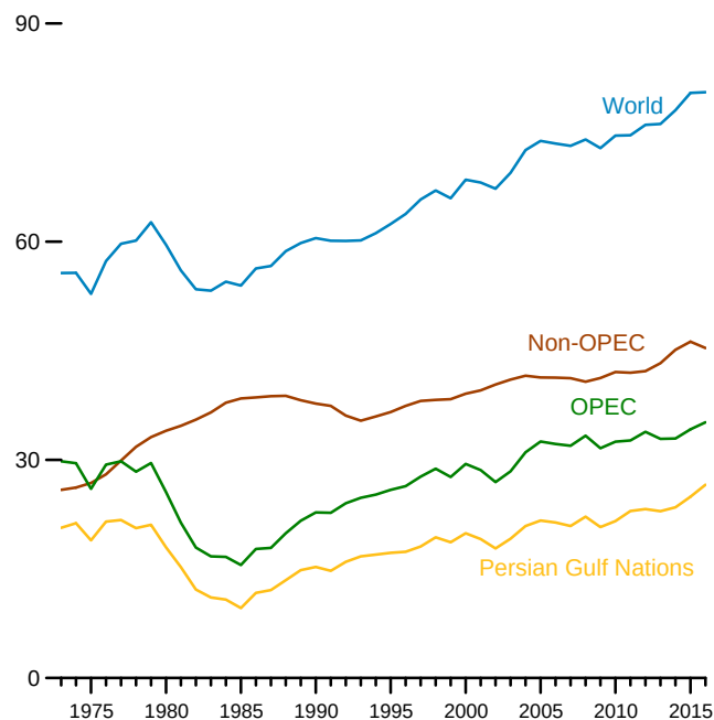
World Production, 1973–2016
