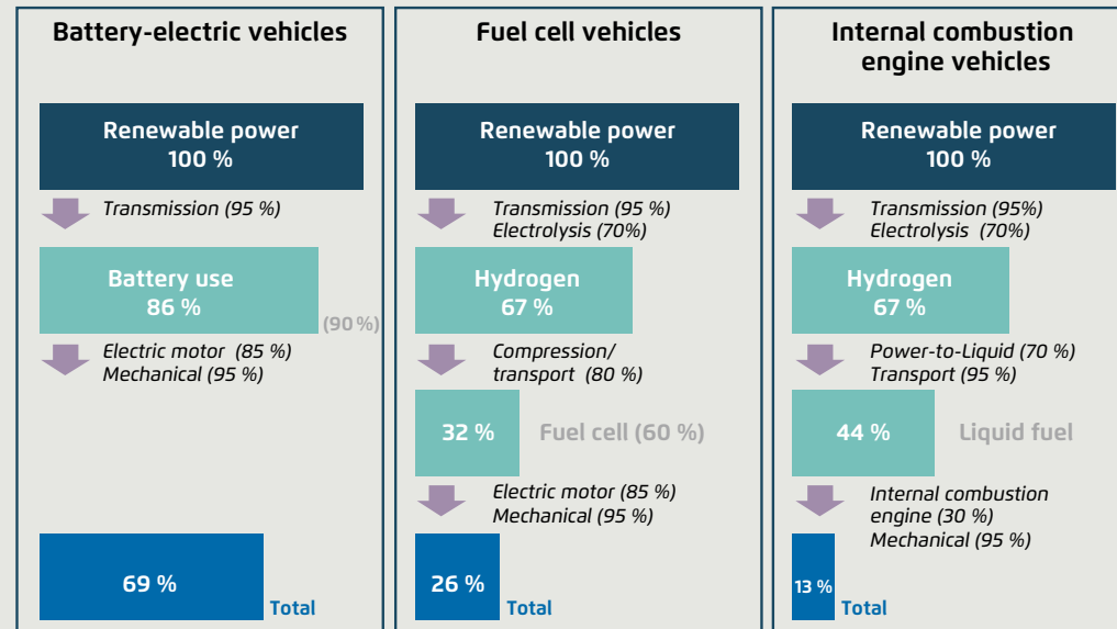
Efficiencies for different electricity-based technology solutions
