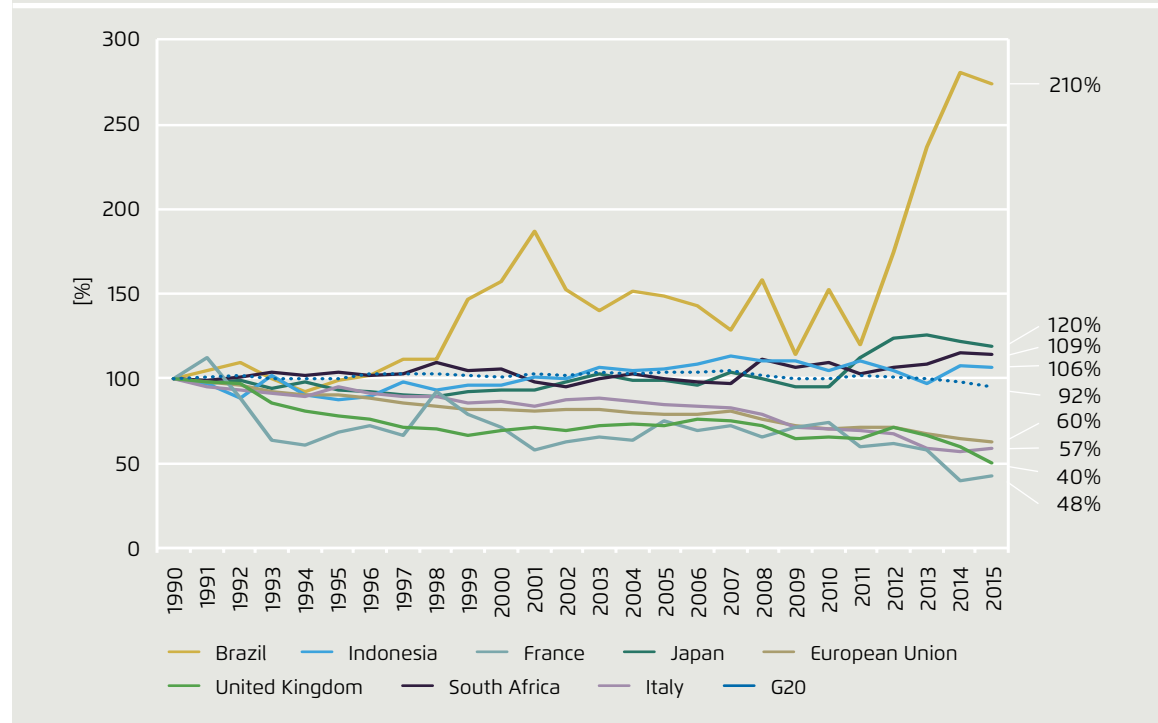
Development of grid emission factors in selected G20 countries
