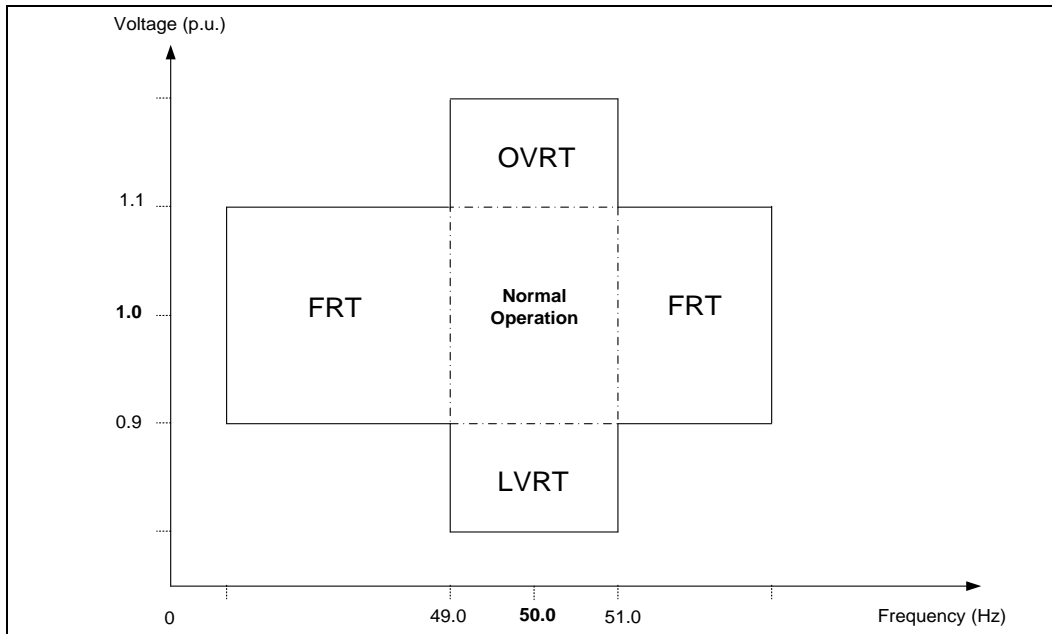
FIGURE 3.2 illustrates typical operation ranges during normal and FRT/HVRT/LVRT conditions (for a 50 Hz system).
