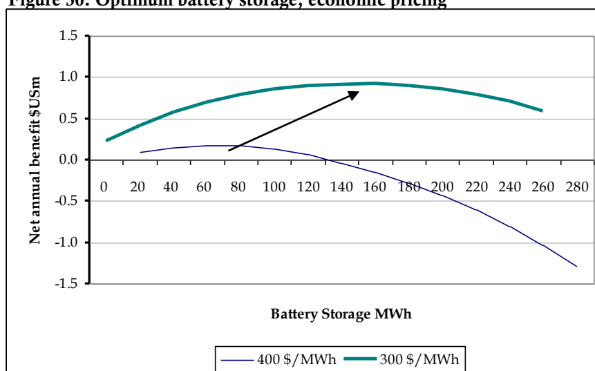
Figure 30: Optimum battery storage, economic pricing
