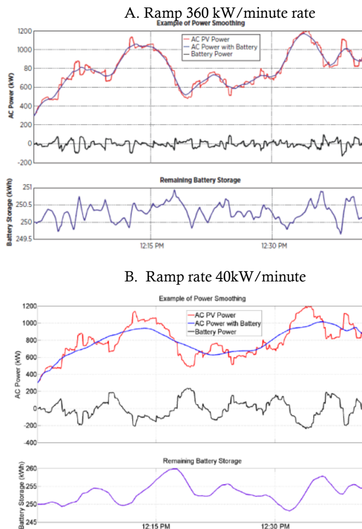
Figure 11: Battery operation for power smoothing at La Ola Solar PV project, Hawaii
