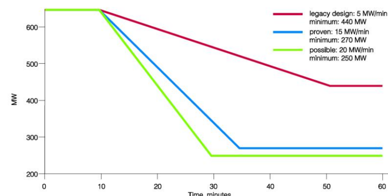
Figure 36: Improvements in ramp rates and minimum load from retrofitting modern control systems
