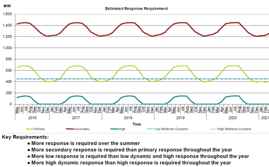
Figure 38: FFR forecasts
