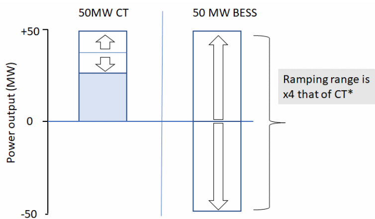
Figure 10: CT v BESS for ramping
