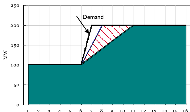
Figure 35: Ramping constraints
