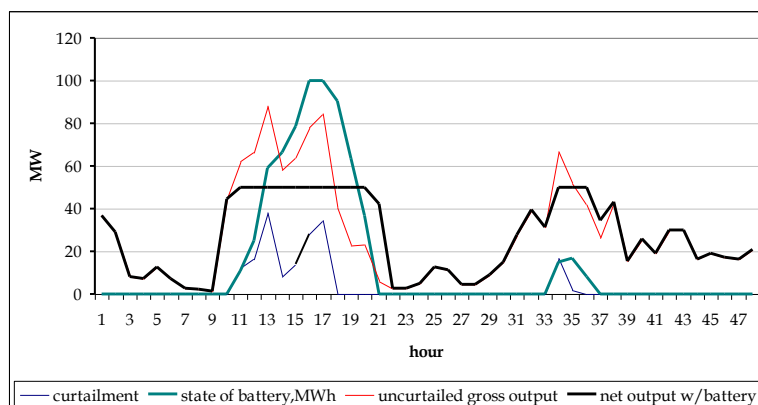
Figure 26: Battery operation
