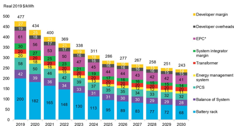
Figure 7: Estimated capital costs, as $/kWh, for fully installed utility scale energy storage system for a 50MW/50MWh system
