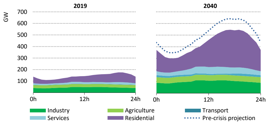
Figure 3.3 ▶ Daily electricity demand in India in 2019 and 2040 in the STEPS
