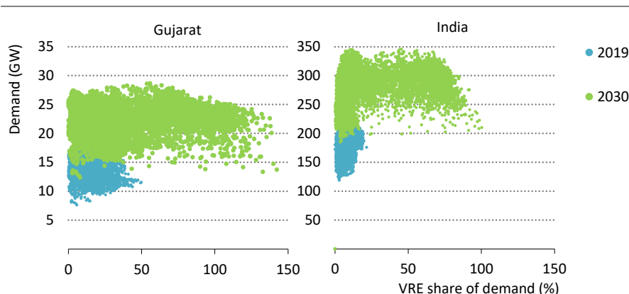
Figure 3.10 ▶ Hourly share of available solar and wind generation as percentage of demand in Gujarat versus India as a whole
