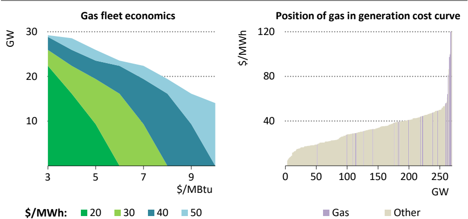
Figure 3.19 ▶ Gas-fired power generation economics under different delivered gas costs and power tariffs, and generating costs in mid-2020
