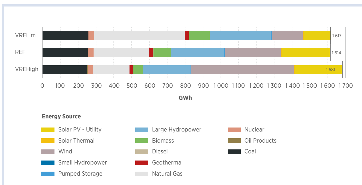
Figure 5-8: Comparison of the Reference scenario, VRELim and VREHigh, 2040
