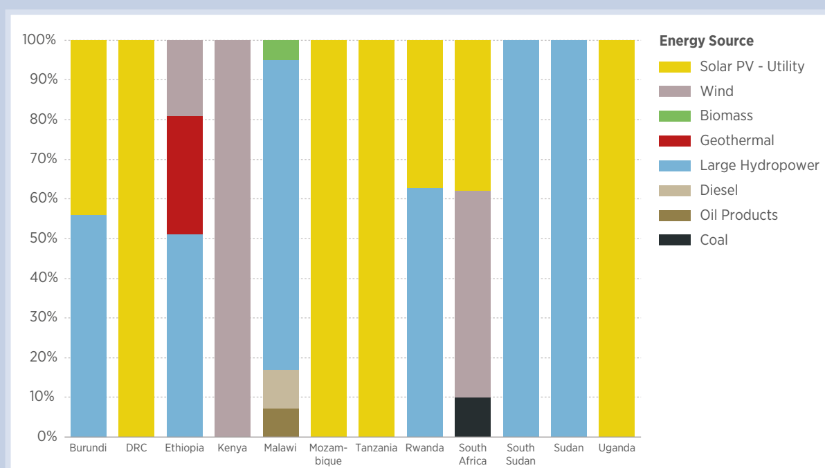
Figure 5-6: Capacity mix of candidate generation projects selected under the Reference scenario, 2015–2025
