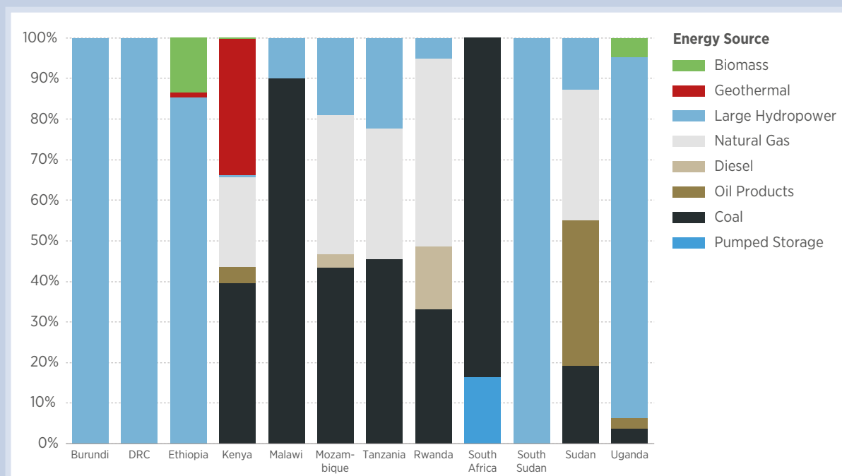
Figure 5-5: Capacity mix of committed generation projects, 2015–2025
