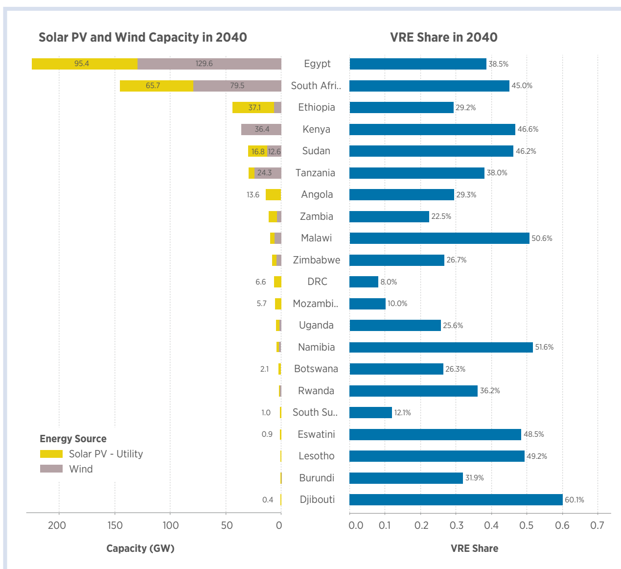
Figure 5-12: VRE capacity and share of generation by country in the Reference scenario, 2040
