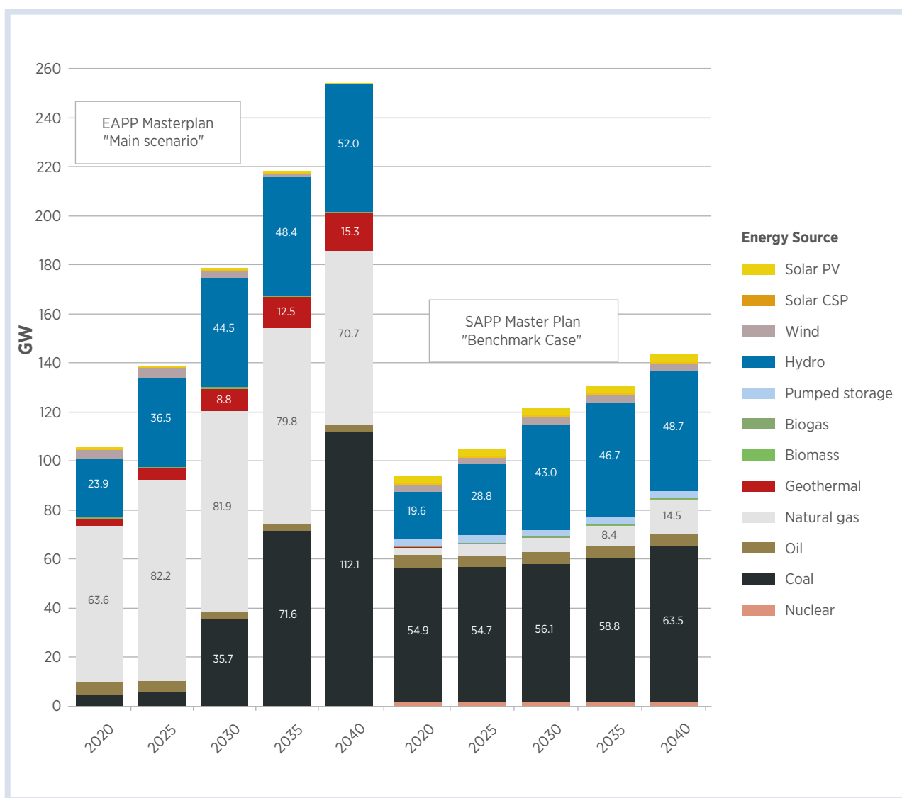
Figure 2-4: EAPP and SAPP's capacity mix until 2040 based on the respective master plans' reference plans 13
