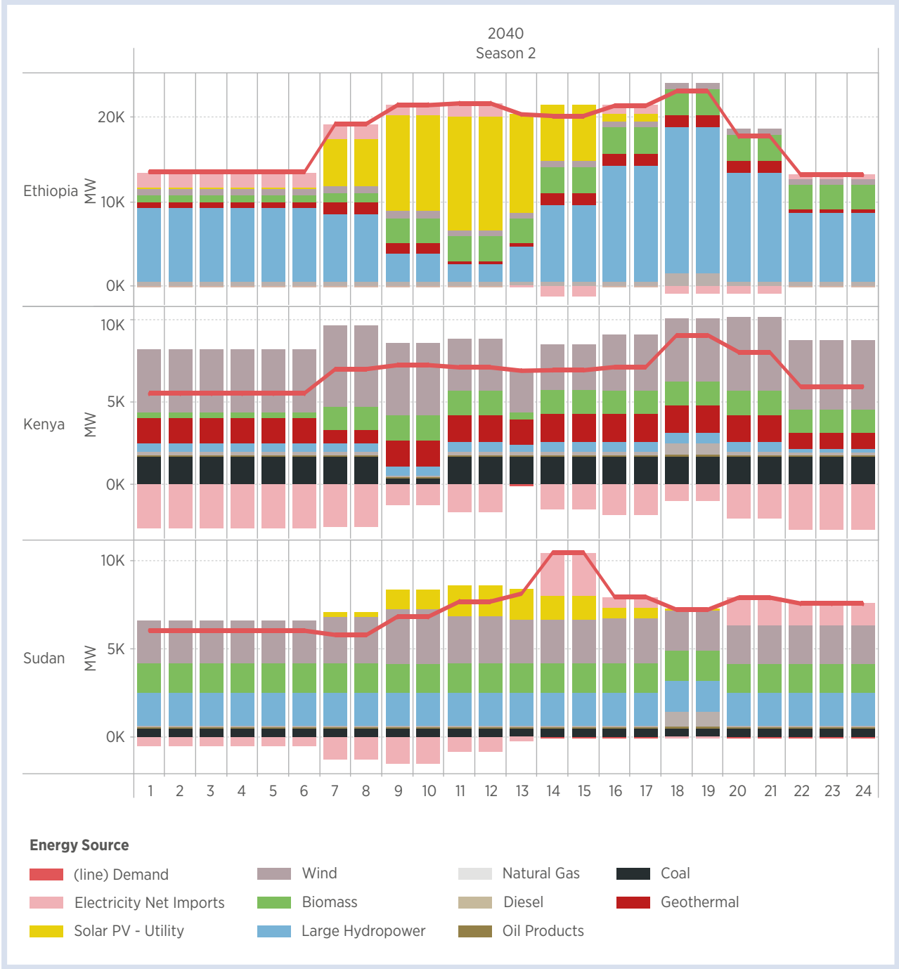
Figure 6-2: Generation mix for Ethiopia, Kenya and Sudan, 2040, season 2, over 24 hours, in SAST (UTC+2:00)
