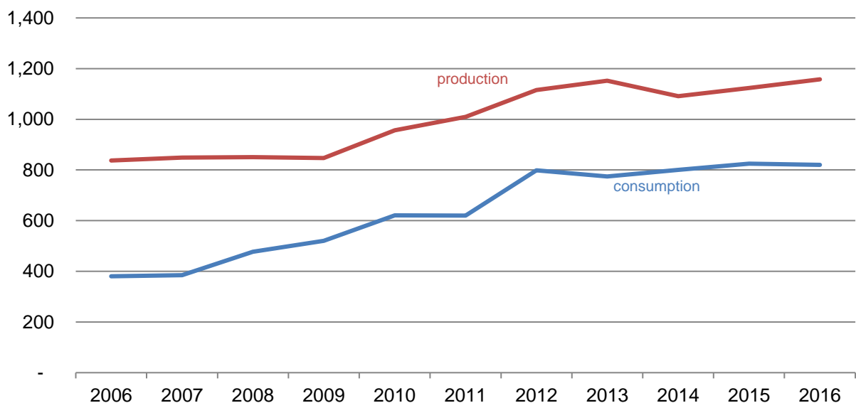
Figure 6: Oman natural gas production and consumption billion cubic feet
